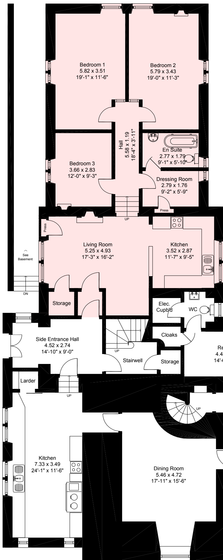
Ground Floor
