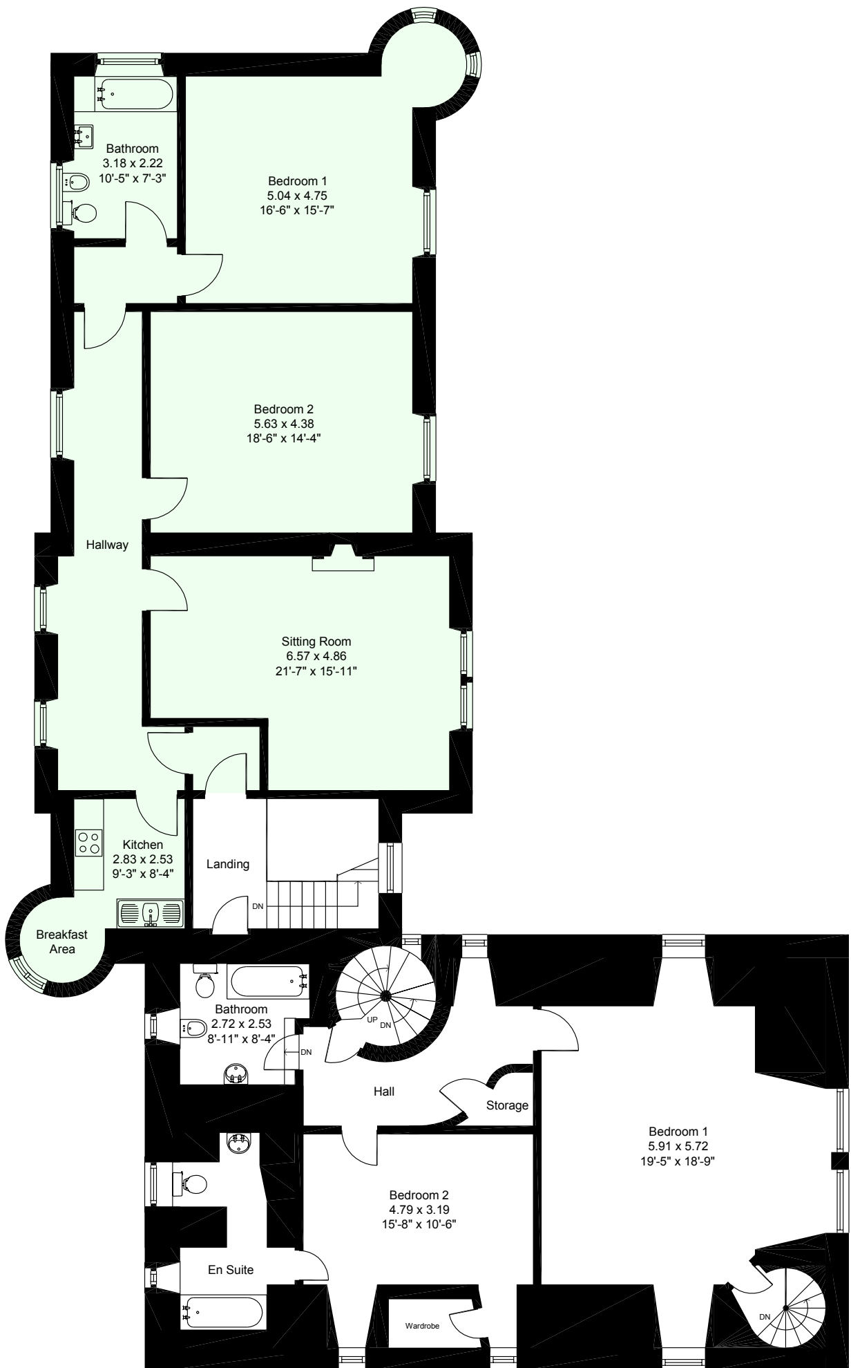
Second Floor
